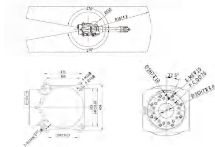
Installation Dimension of Base Flange Dimensions
