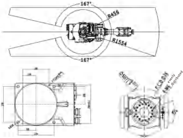
Installation Dimension of Base Flange Dimensions
