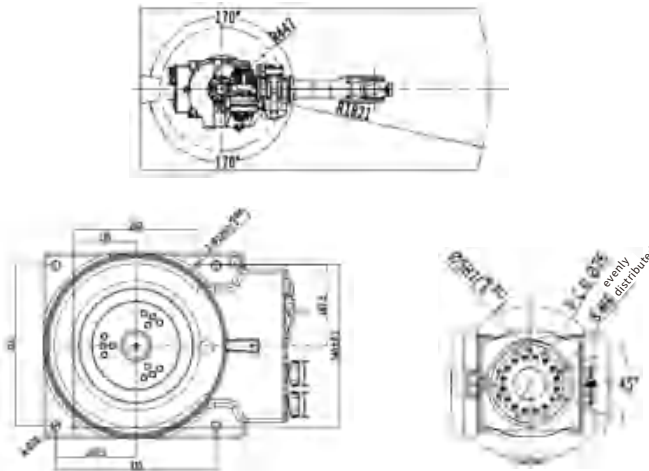
Installation Dimension of Base Flange Dimensions
