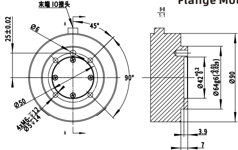
Flange Mounting Diagram
