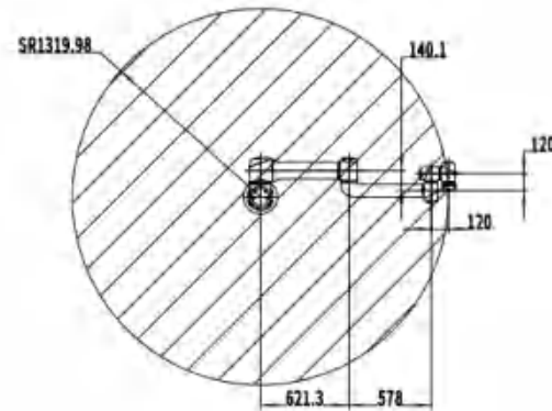
CRP-RC13-10
