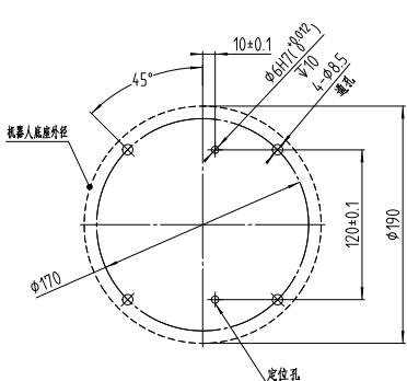
CRP-RC13-10/CRP-RC18-05
