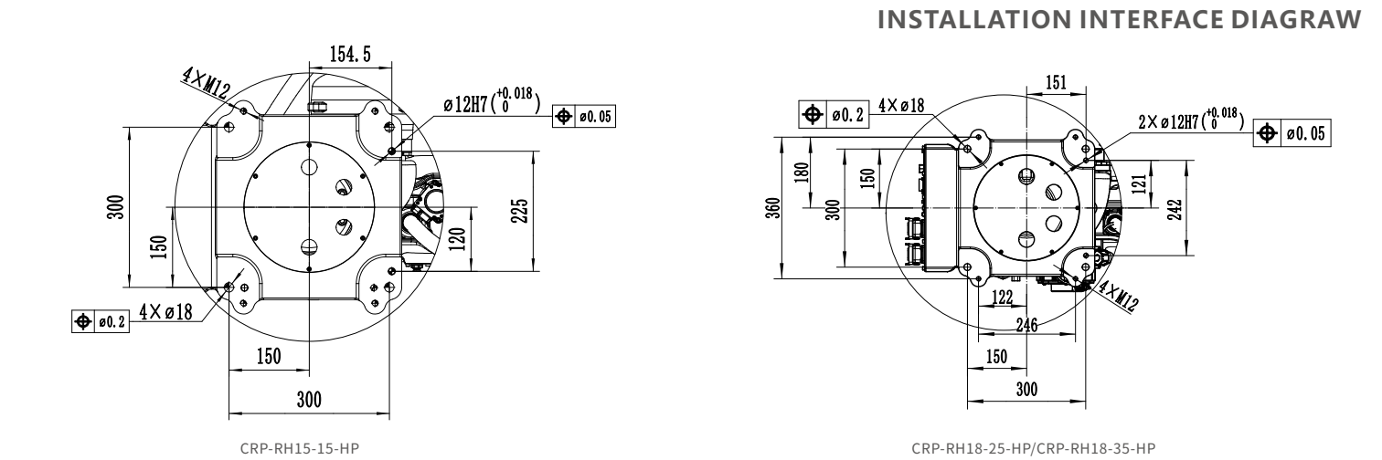
Base mounting dimension
